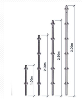
Vertical standard
